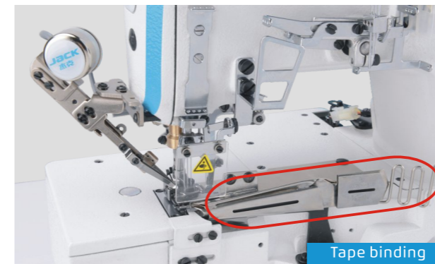
Tape binding
